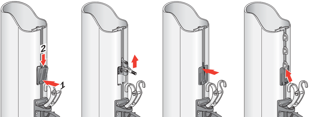
Remove sail entry to install MDS cars. 1 Push in 2 Push down
