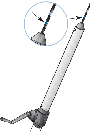
Mark the backstay with two pieces of tape at normal- and maximum load. The tape markers will enable you to re-tension the stay accurately.
