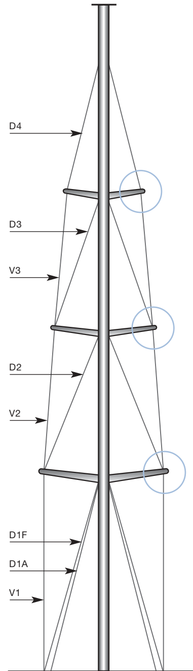
Linked rigging.
