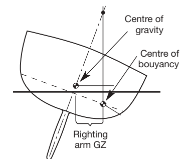
Righting moment = GZ \times \text{displacement} .
